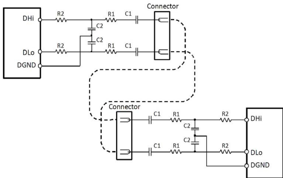
FIGURE 59. ISL94212 DAISY CHAIN CIRCUIT IMPLEMENTATION
