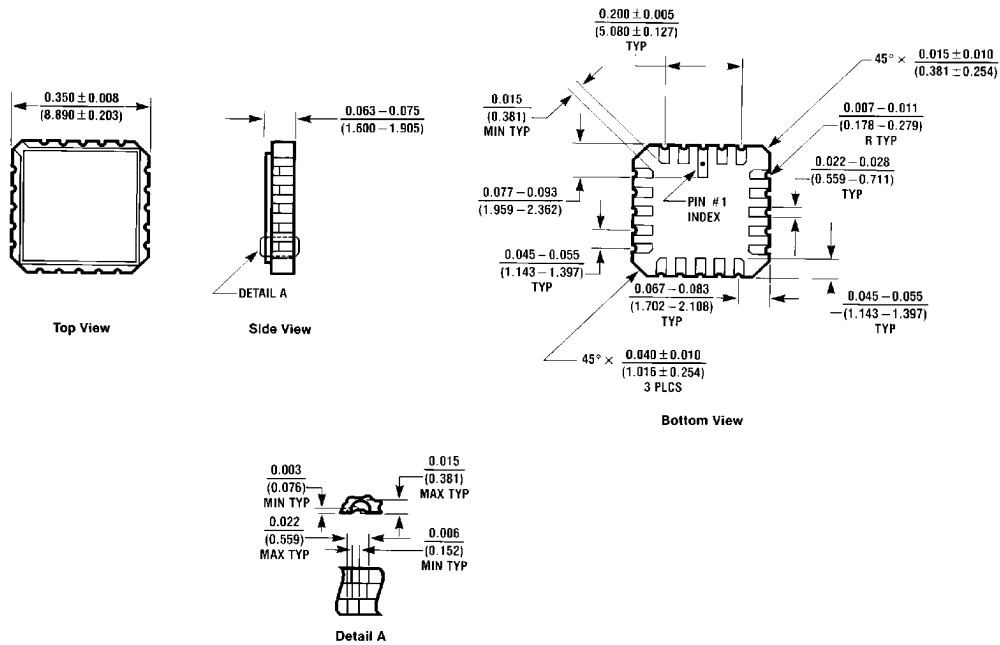
Ceramic Leadless Chip Carrier Package (E) Order Number DM54LS260E NS Package Number E20A
