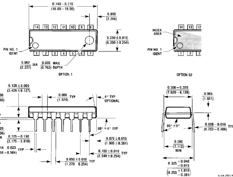
14-Lead Molded Dual-In-Line Package (N) Order Number DM74LS260N NS Package Number N14A
