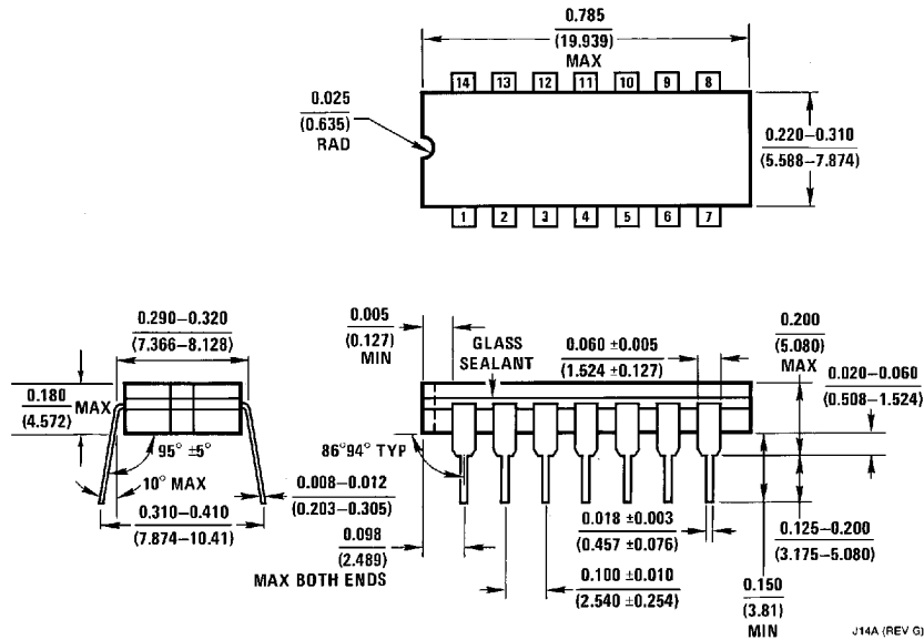
14-Lead Ceramic Dual-In-Line Package (J) Order Number DM54LS260J NS Package Number J14A
