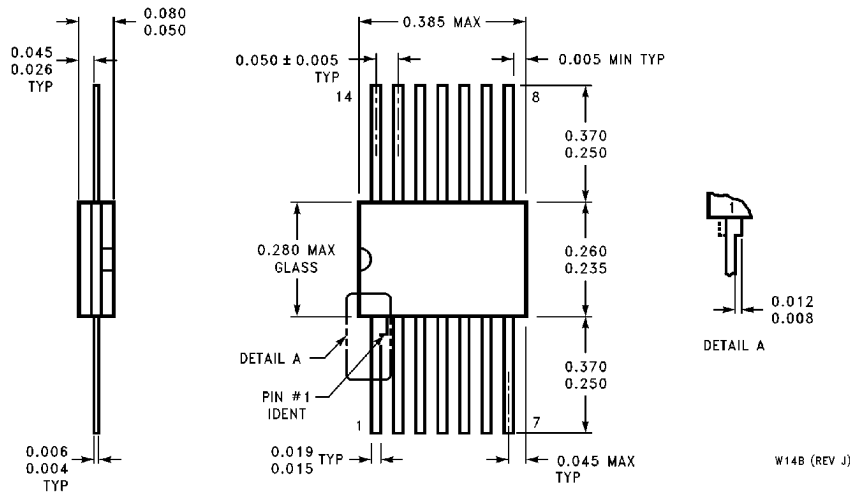
14-Lead Ceramic Flat Package (W) Order Number DM54LS260W NS Package Number W14B
