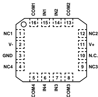
ISL43140 (QFN) TOP VIEW
