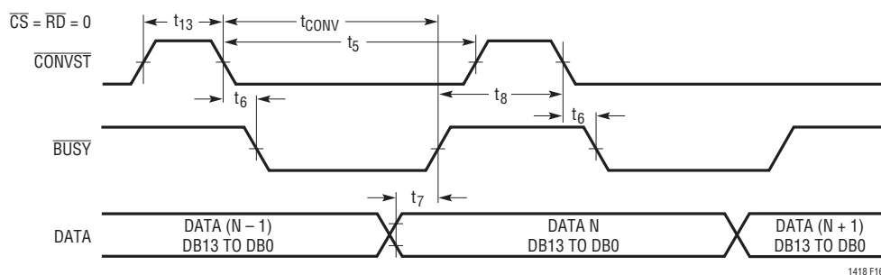
Figure 16. Mode 1b. \overline{\text{CONVST}} Starts a Conversion. Data Outputs Always Enabled ( \overline{\text{CONVST}} = \text{high} )
