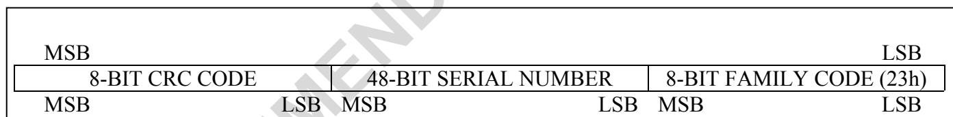
Figure 3. 64-BIT LASERED ROM
