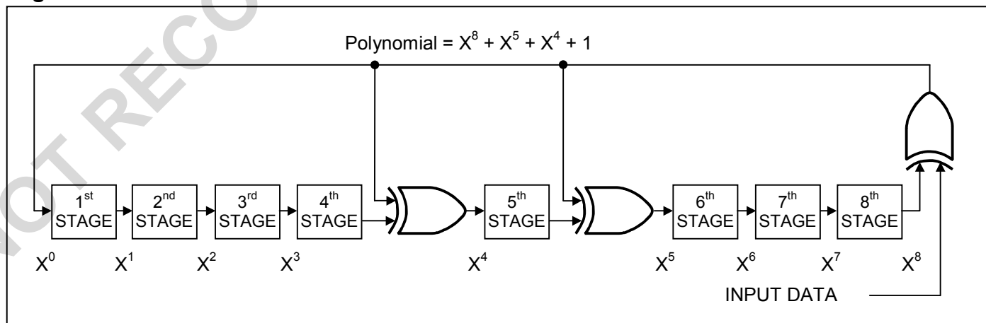
Figure 4. 1-Wire CRC GENERATOR
