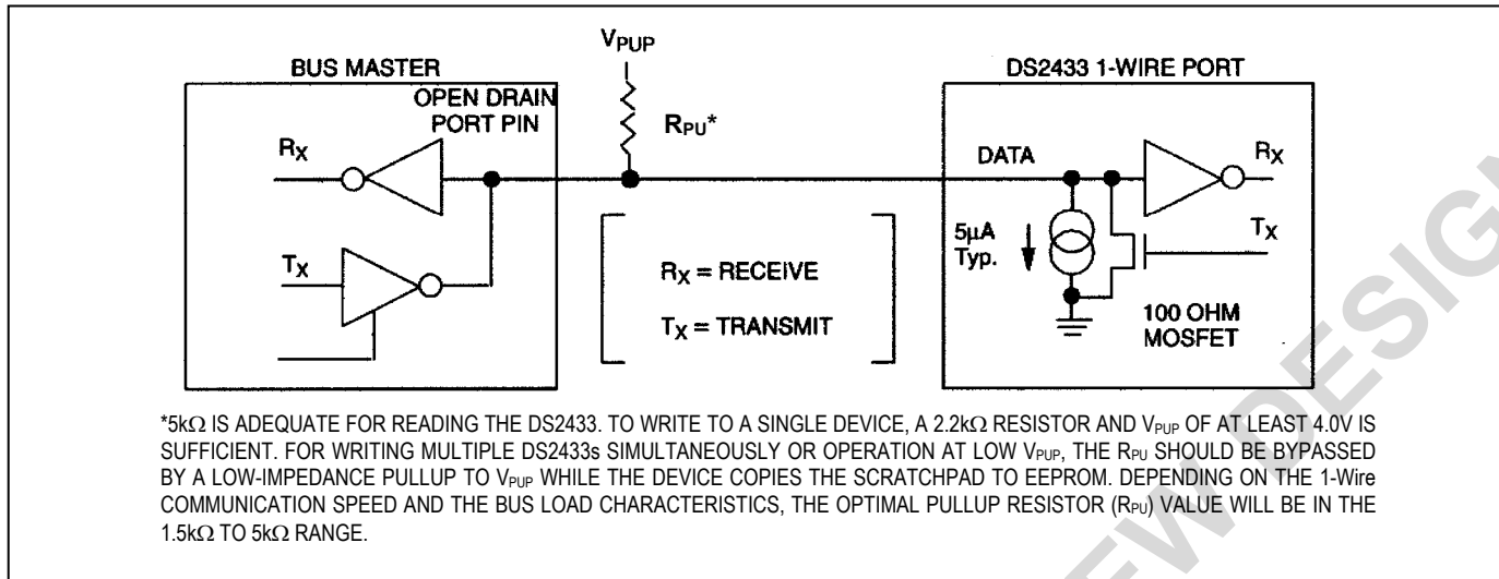
Figure 8. HARDWARE CONFIGURATION
