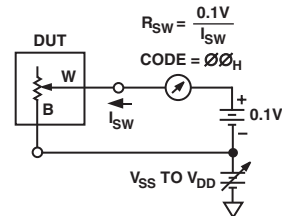
Test Circuit 8. Incremental On Resistance
