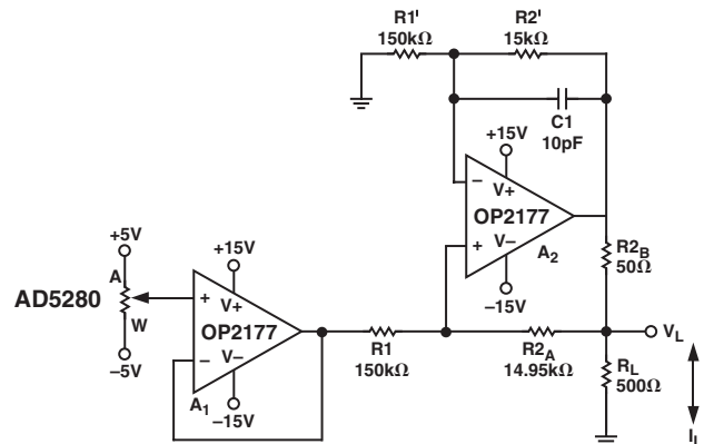
Figure 20. Programmable Bidirectional Current Source
