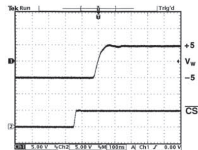
TPC 24. Large Signal Settling Time
