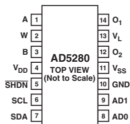
AD5280 PIN CONFIGURATION
