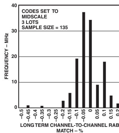
TPC 27. Channel-to-Channel Resistance Matching (AD5282)
