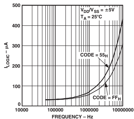
TPC 21. V_{\text{LOGIC}} Supply Current vs. Frequency
