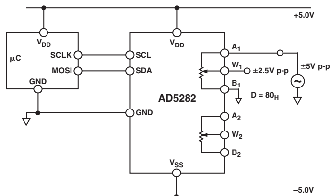
Figure 13. Bipolar Operation from Dual Supplies
