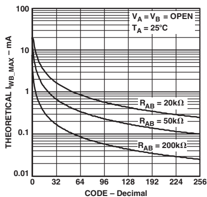
TPC 26. I_{\text{MAX}} vs. Code
