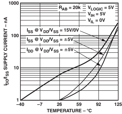
TPC 11. Supply Current vs. Temperature
