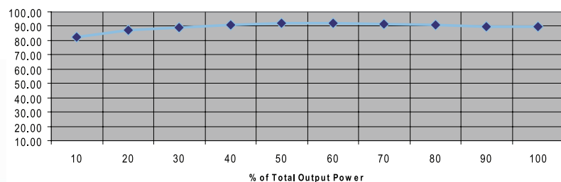
230 Vac Efficiency
