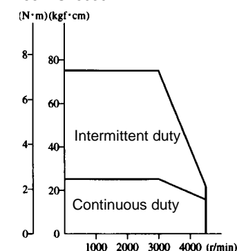
R88M-U75030HA (N·m)(kgf·cm)
