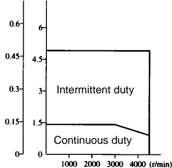
R88M-U30030LA (N·m)(kgf·cm)
