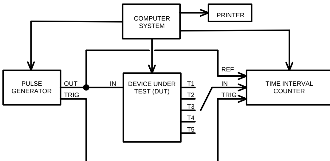
Test Setup
