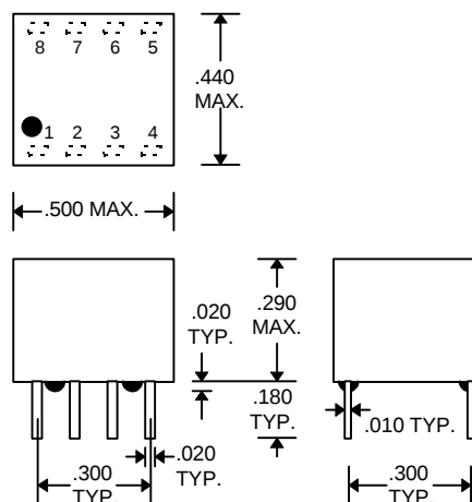
DDU8C-xxM (Military DIP)
