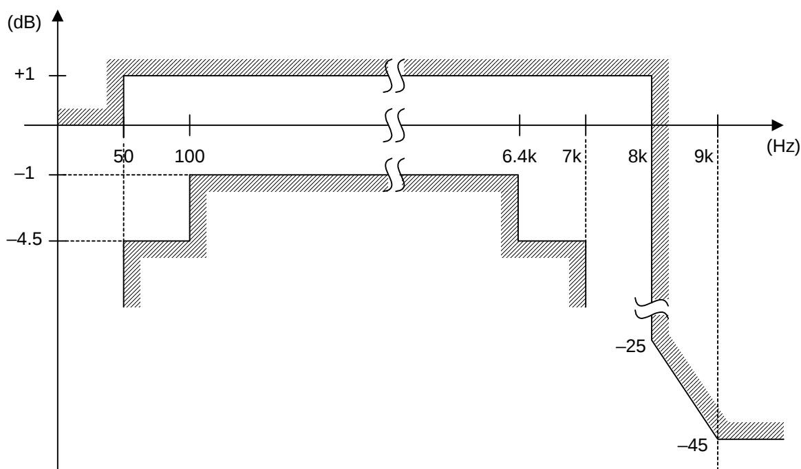
Figure 1. Transmit and Receive Path Attenuation Distortion—Wideband Mode
