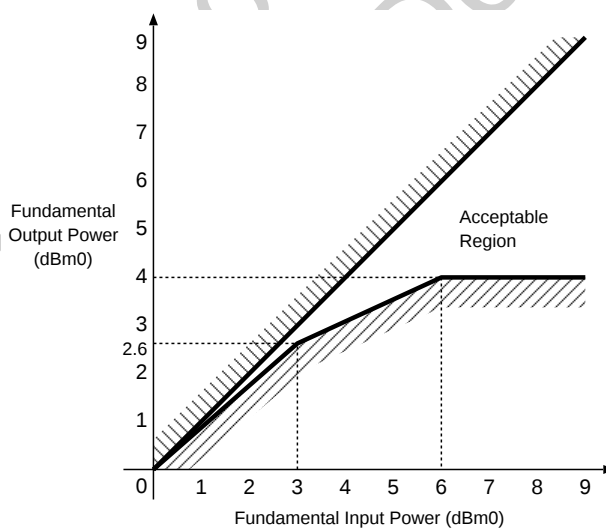
Figure 4. Overload Compression Performance
