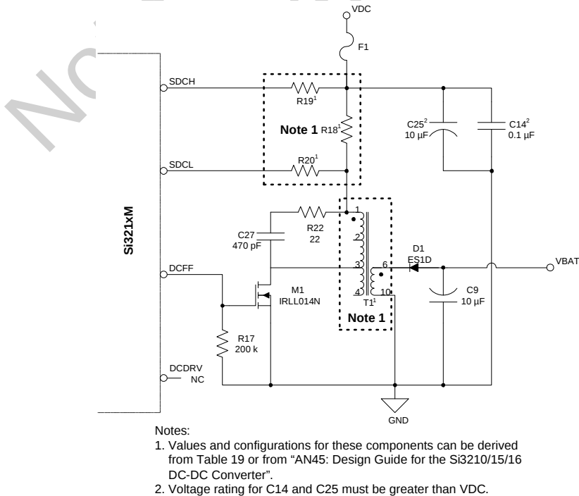
Figure 14. Si321xM MOSFET/Transformer DC-DC Converter Circuit
