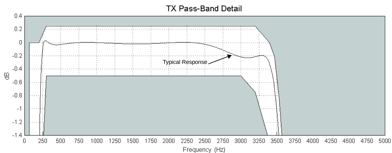
Figure 5. Transmit Path Frequency Response—Narrowband Mode
