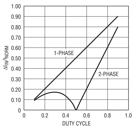
Figure 24. Normalized Input Peak-to-Peak Ripple Current
