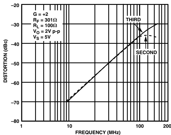
TPC 9. Distortion vs. Frequency; G = +2 ; V_S = 5\text{ V}
