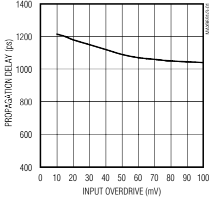
WORST-CASE PROPAGATION DELAY vs. INPUT OVERDRIVE
