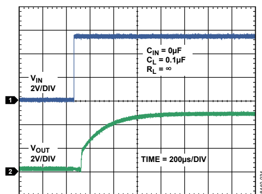
Figure 25. ADR3450 Start-Up Response
