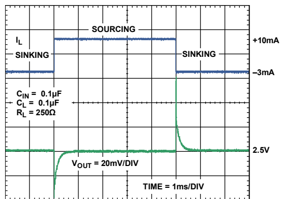
Figure 29. ADR3425 Load Transient Response
