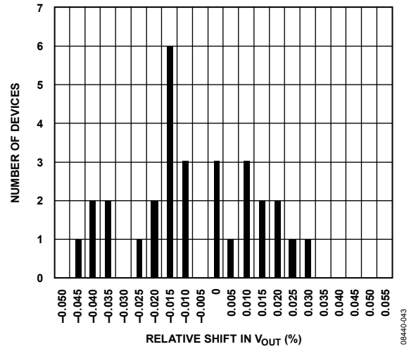
Figure 36. Output Voltage Drift Distribution After Reflow (SHR Drift)
