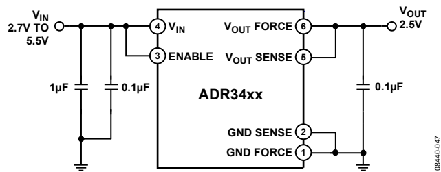
Figure 40. Basic Reference Connection
