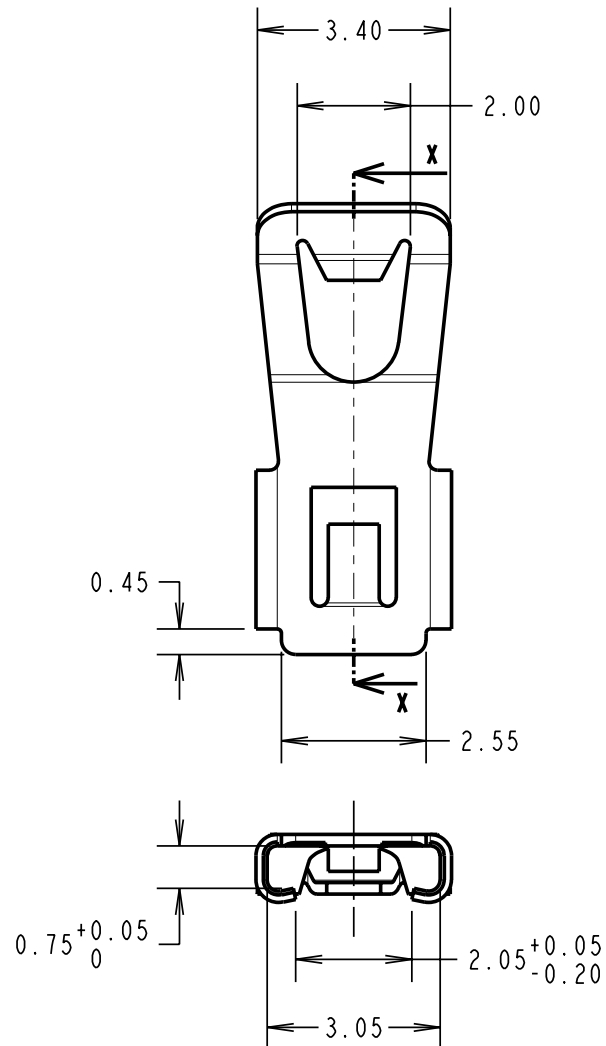
SECTION X-X
