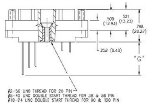
TYPICAL RECEPTACLE WITH LOCKNUT AND POLARIZING SOCKETS
