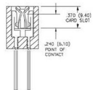
SECTION THROUGH CONTACT POSITION
