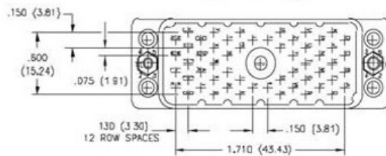
56 PIN PLUG
