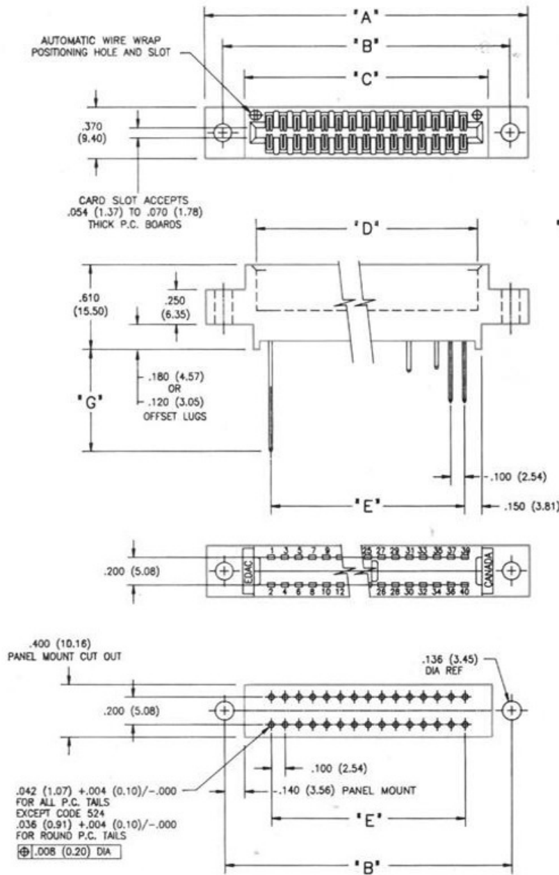
CONNECTOR MOUNTING PATTERN
