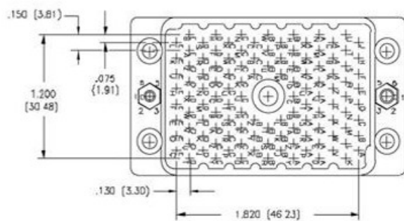
120 PIN PLUG
