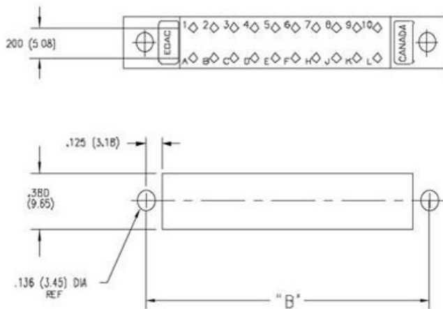
CONNECTOR MOUNTING PATTERN PANEL MOUNT CUT OUT
