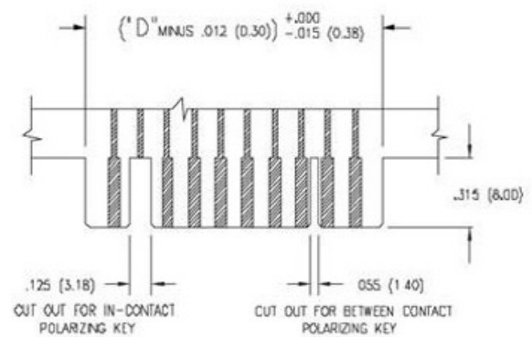
RECOMMENDED DAUGHTER BOARD
