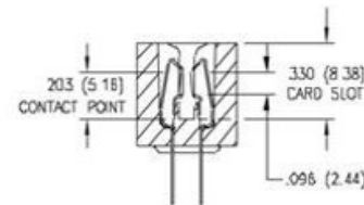
SECTION THROUGH CONTACT POSITION
