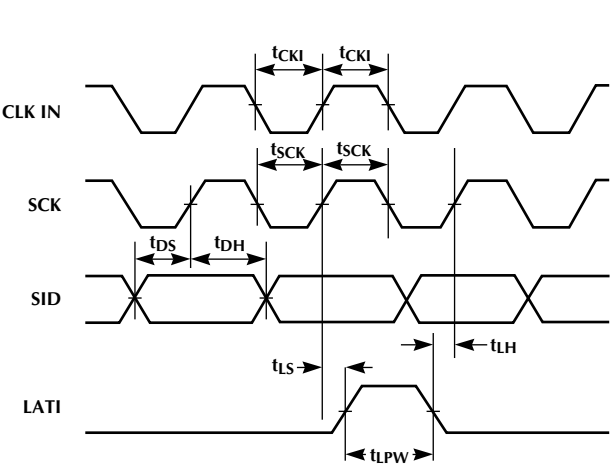
Figure 1. Serial Interface Timing.
