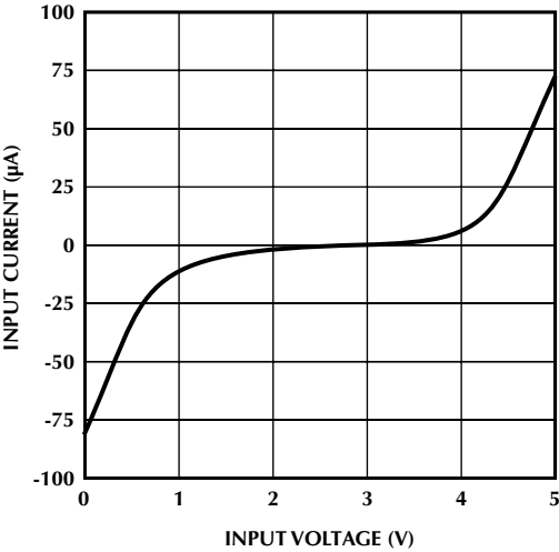
Figure 2. CLK IN Input Current vs. Input Voltage.
