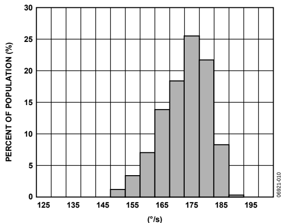
Figure 10. Measurement Range
