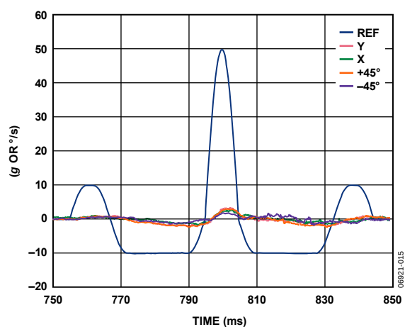
Figure 15. g and g x g Sensitivity for a 50 g, 10 ms Pulse
