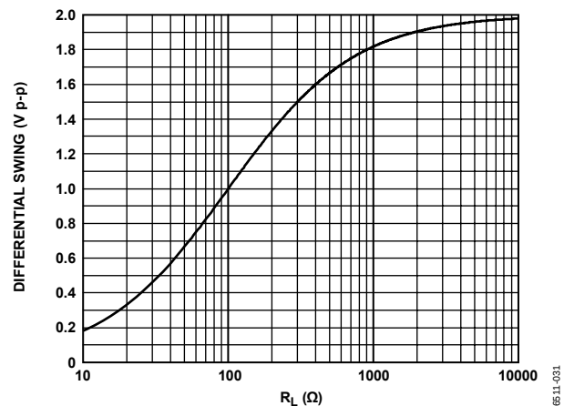
Figure 31. Relationship Between the AC Swing-Limiting Resistor and the Peak-to-Peak Voltage Swing with 50 \Omega Bias-Setting Resistors
