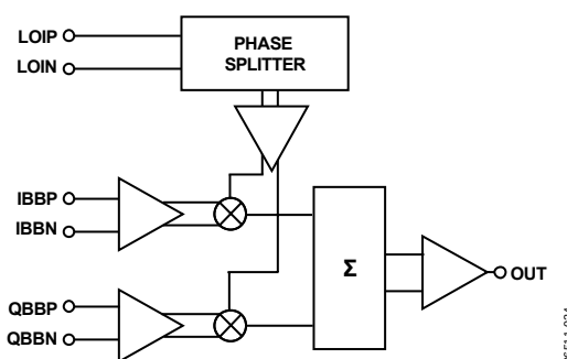
Figure 24. Block Diagram
