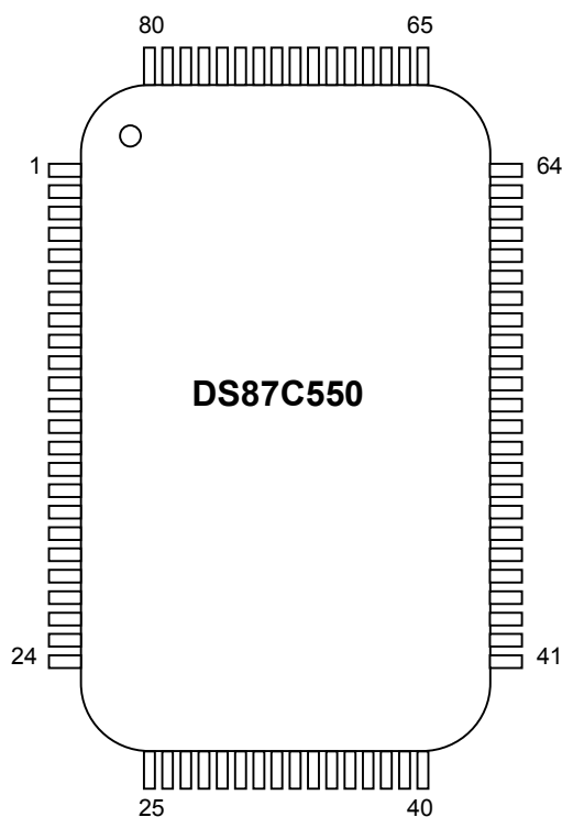
80-Pin PQFP
