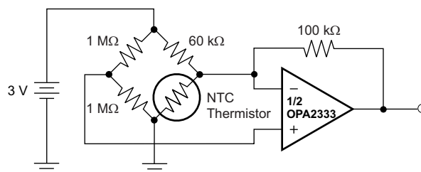
Figure 33. Thermistor Measurement
