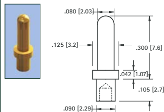
.080 (2.0) PIN - SWAGE MOUNT
