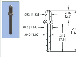
.040 (1.0) HOLLOW PIN - SWAGE MOUNT
