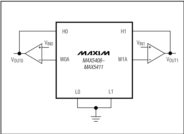
Figure 6. Gain Control
