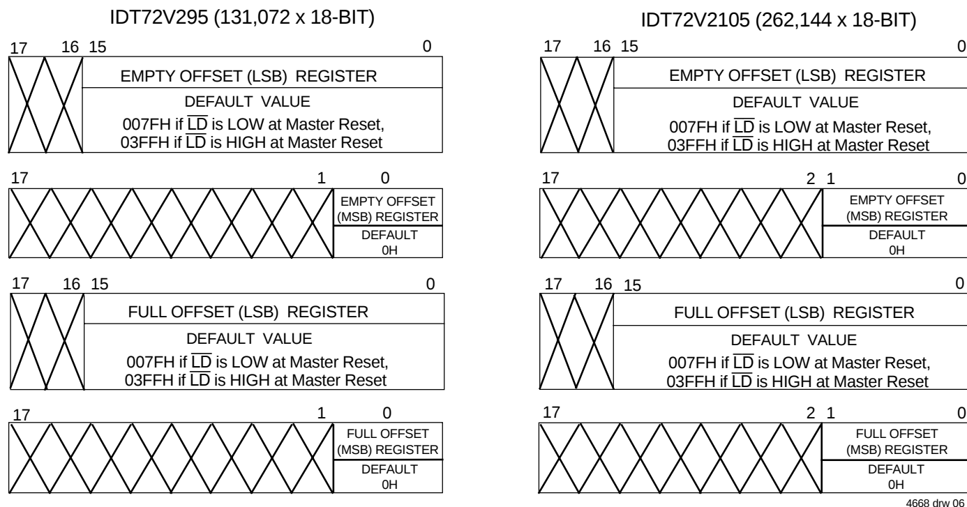
Figure 3. Offset Register Location and Default Values
