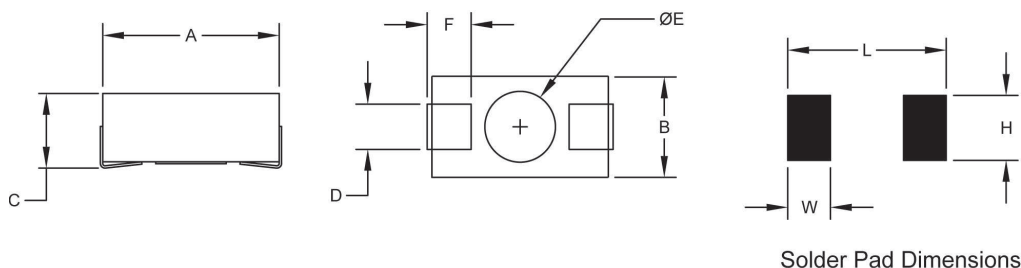
Solder Pad Dimensions
