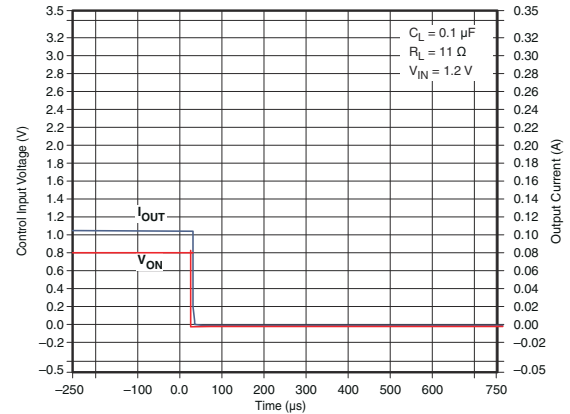
Figure 7-54. t_{OFF} Response
