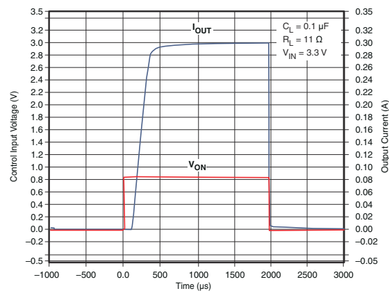
Figure 7-42. t_{ON} Response
