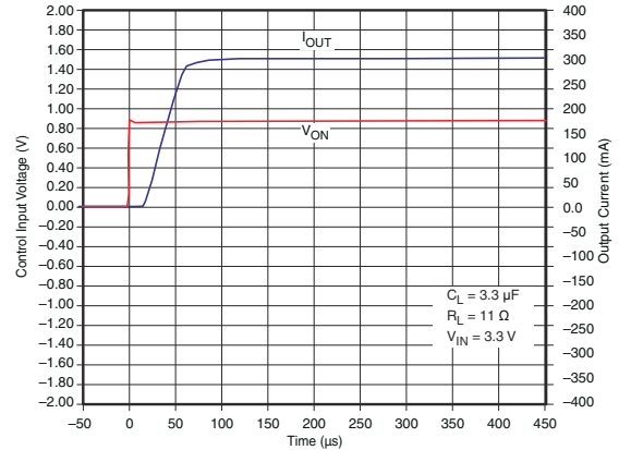
Figure 7-20. t_{ON} Response
