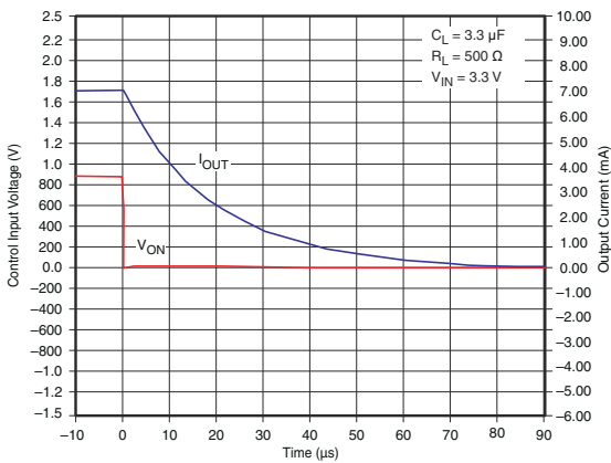
Figure 7-27. t_{OFF} Response
