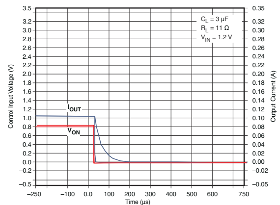
Figure 7-56. t_{OFF} Response
