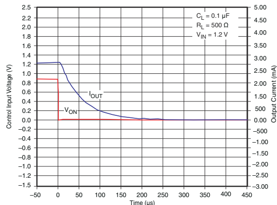
Figure 7-29. t_{OFF} Response
