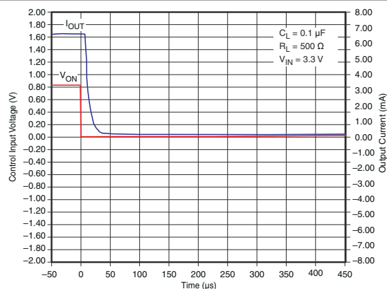
Figure 7-33. t_{OFF} Response
