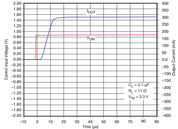
Figure 7-18. t_{ON} Response
