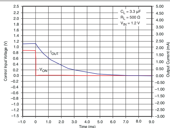
Figure 7-31. t_{OFF} Response
