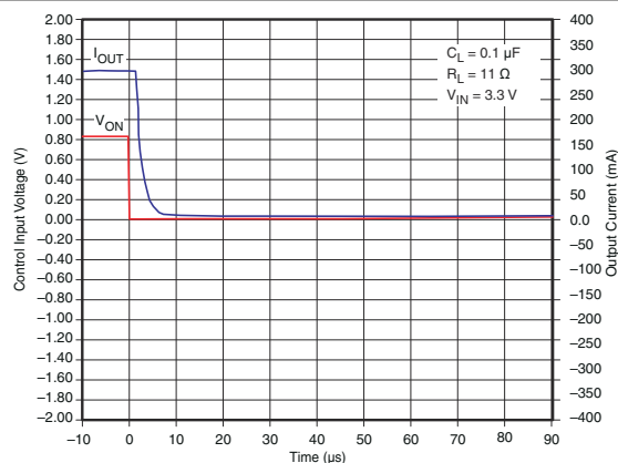
Figure 7-34. t_{OFF} Response
