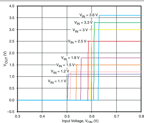
Figure 7-10. ON-Input Threshold
