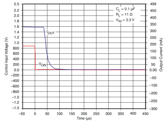
Figure 7-26. t_{OFF} Response
