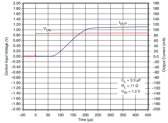
Figure 7-24. t_{ON} Response
