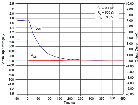
Figure 7-25. t_{OFF} Response
