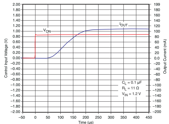
Figure 7-22. t_{ON} Response
