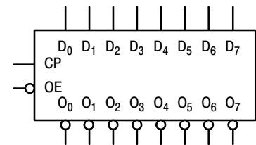
Figure 2. LOGIC SYMBOL
