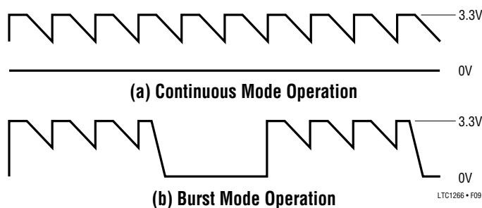
Figure 9. C_T Waveforms
