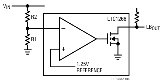
Figure 6. Low-Battery Comparator
