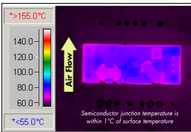
Figure 6: Thermal plot of converter at 15 amp load current with 55°C air flowing at the rate of 200 LFM. Air is flowing across the converter sideways from pin 3 to pin 1 (nominal input voltage).
