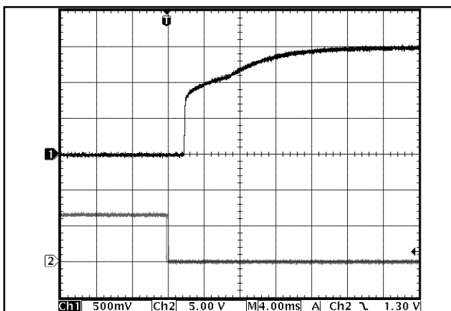
Figure 10: Turn-on transient at zero load (4 ms/div). Ch 1: V_{out} (500mV/div). Ch 2: ON/OFF input (5V/div)
