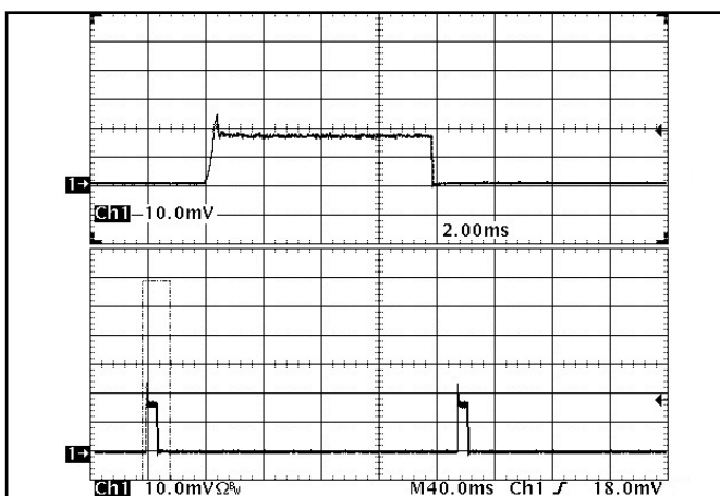
Figure 18: Load current (10A/div) as a function of time when the converter attempts to turn on into a 10 m \Omega short circuit. Top trace (2.0ms/div) is an expansion of the on-time portion of the bottom trace.
