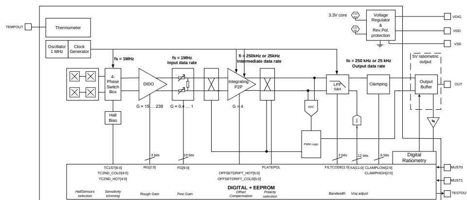
Figure 1: Block diagram
