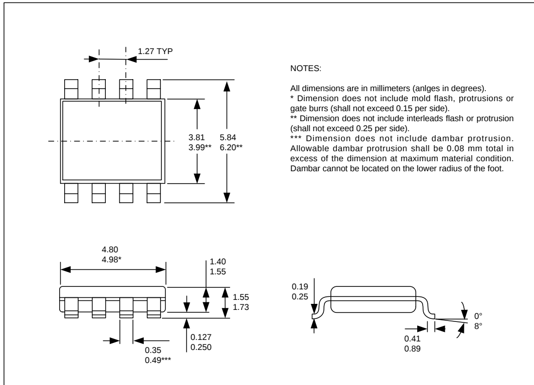
Figure 9: Package dimensions
