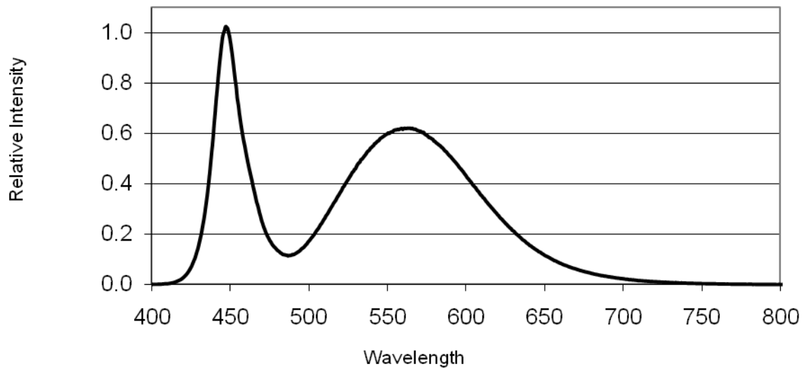
Figure 5: Typical Cool White Color Spectrum
