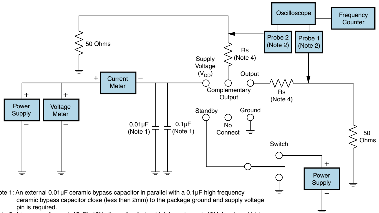
Test Circuit for Standby (Pad 1) and Complementary Output
