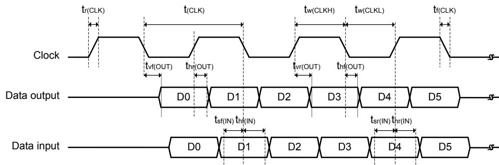
Figure 50. OctoSPI timing diagram - DTR mode
