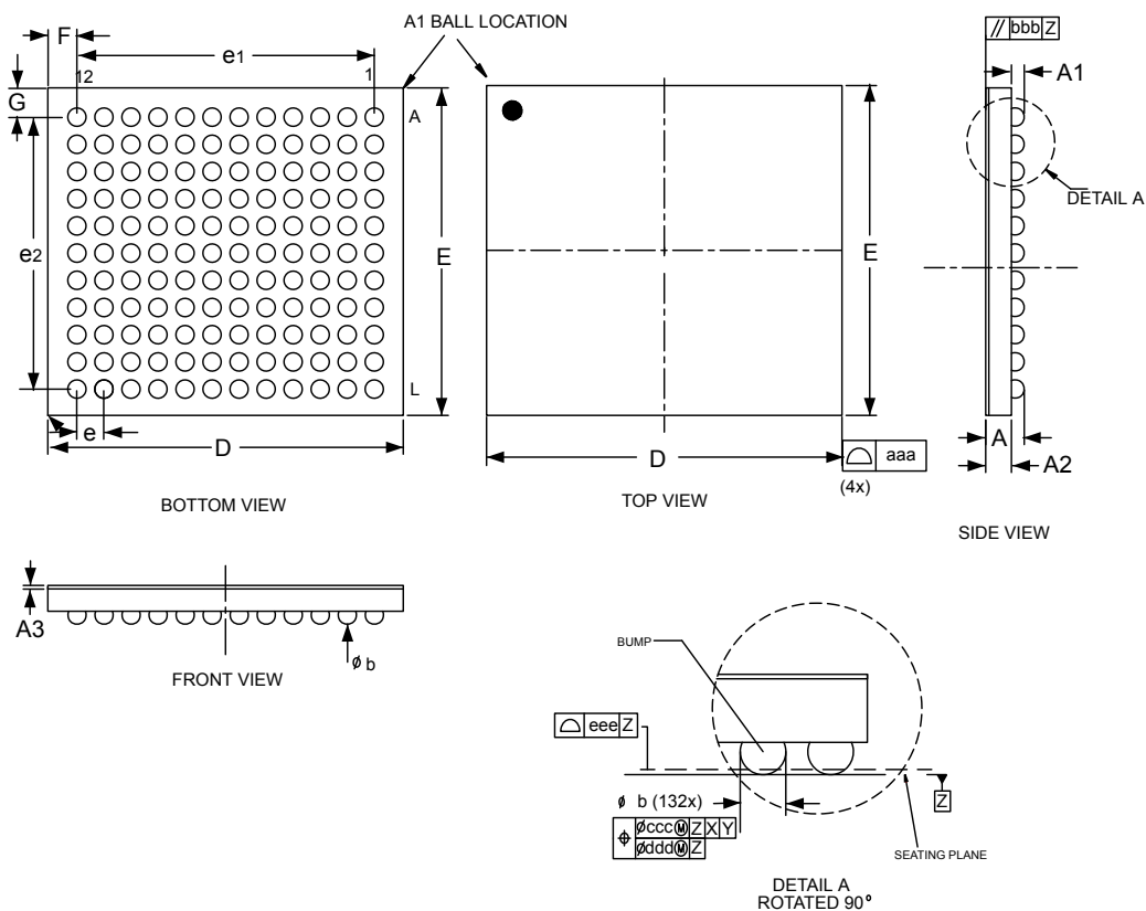
Figure 91. WLCSP132 - Outline
