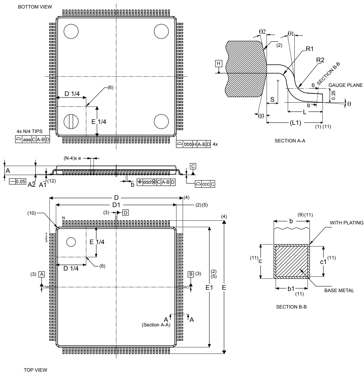
Figure 94. LQFP144 - Outline (15.)
