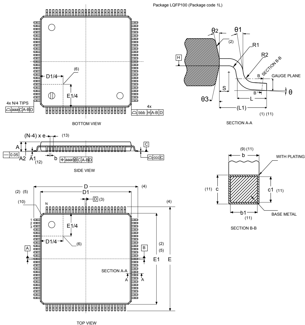
Figure 85. LQFP100 - Outline (15.)
