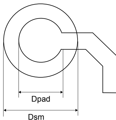
Figure 107. UFBGA169 - Recommended footprint
