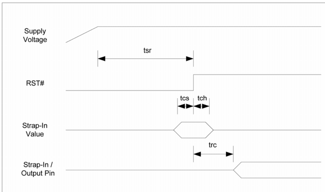
Figure 16. Reset Timing
