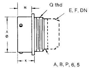
Crimp KPSE00/MS3120
