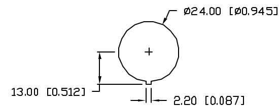
PANEL CUTOUT
