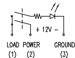
INTERNAL CIRCUIT
