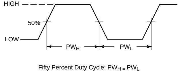
Figure 9. Input/Output Duty Cycle
