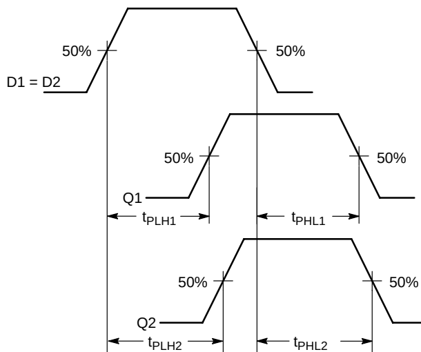
Figure 29. Within Device Skew
