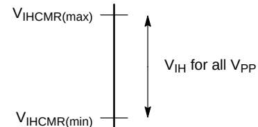
Figure 13. Common Mode Range
