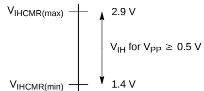
Figure 14. MC100LVEL14 Common Mode Range
