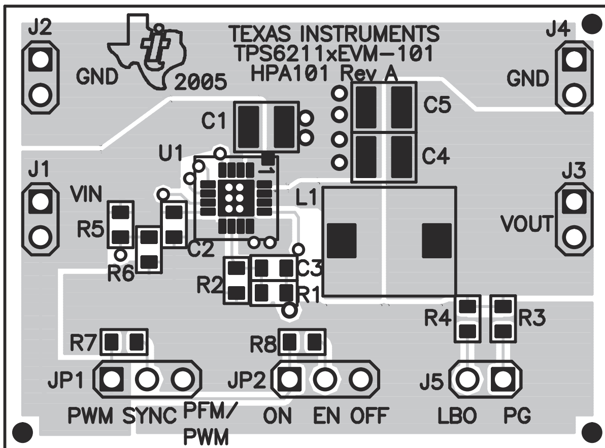
Figure 3-1. Assembly Layer
