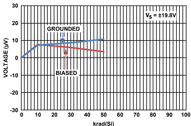
FIGURE 58. V_{OS} SHIFT vs LOW DOSE RATE RADIATION
