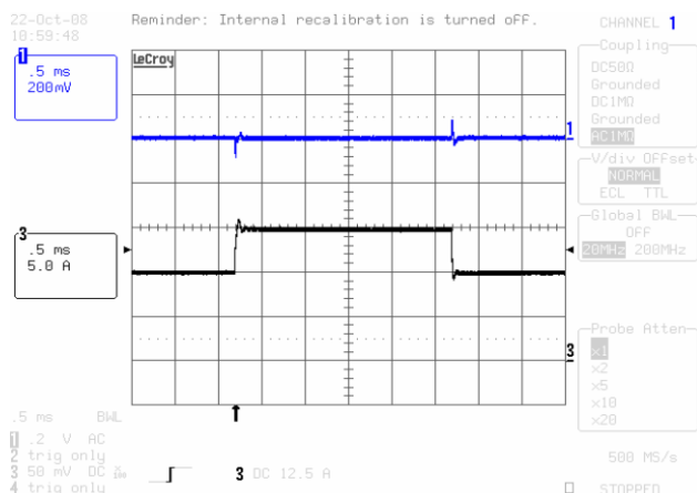
Figure 12. Vin=12V, Vout=0.5V
