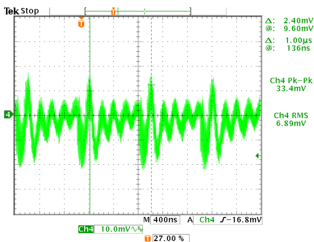
Figure 40. Input Voltage Noise with Interleave
