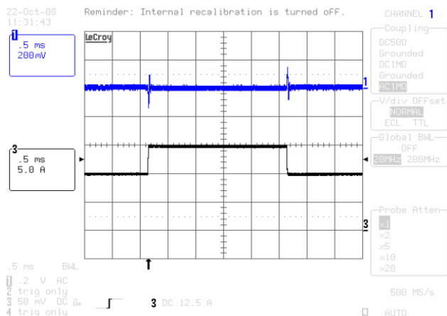
Figure 11. Vin=12V, Vout=2.5V
