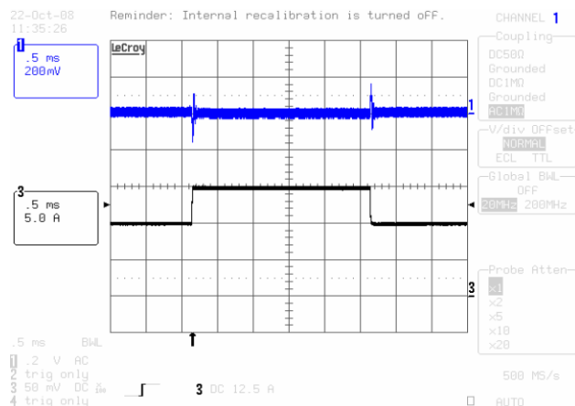
Figure 10. Vin=12V, Vout=5.0V
