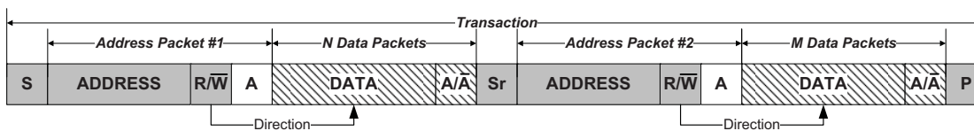
Figure 19-7. Combined Transaction
