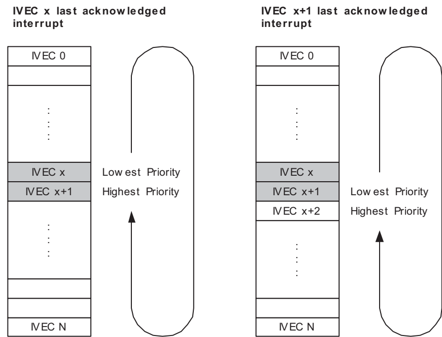
Figure 11-4. Round-robin Scheduling
