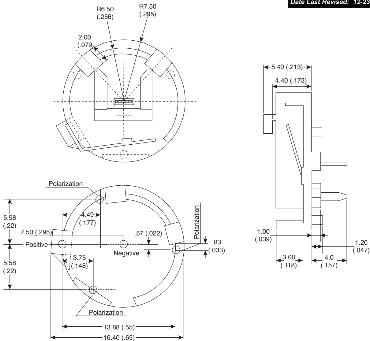
PCB Layout
