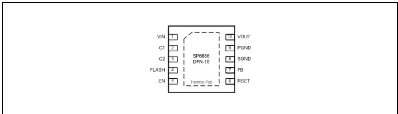
PIN ASSIGNMENT
