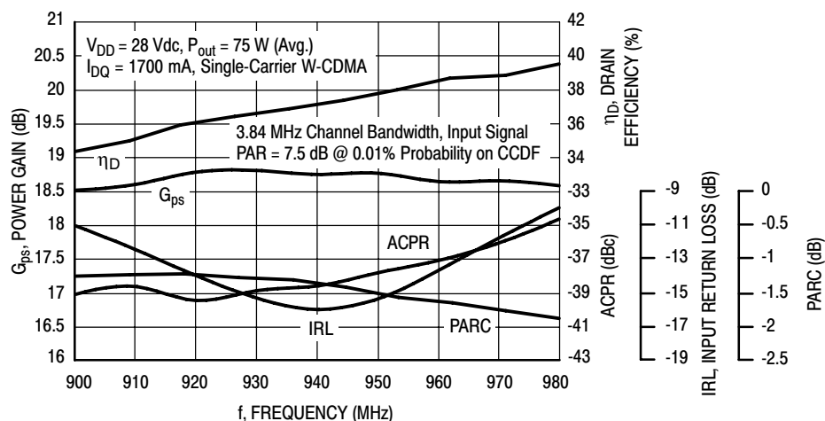
Figure 2. Output Peak-to-Average Ratio Compression (PARC) Broadband Performance @ P_{out} = 75 Watts Avg.
