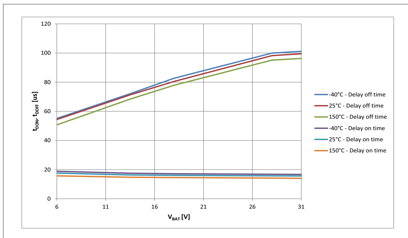
Figure 29 Typical t_{ON} , t_{OFF} vs. V_{BAT} @ V_{IN} = 5V ; T_J = -40 \dots 150^\circ C
