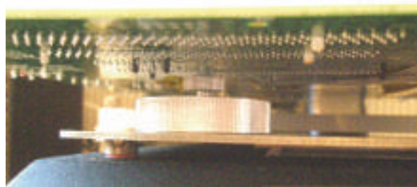
BH-1000 Post-Rail Board Holder. Includes: 4 posts, 2 rails with sliding clips, 4 support pins and flat-head support
