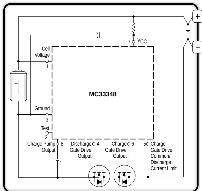
Typical One Cell Smart Battery Pack
