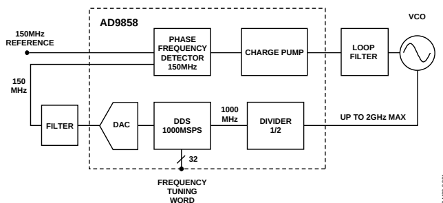
Figure 1. AD9858 Fractional Divider Evaluation Board
