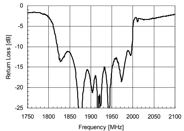
Figure 8. Antenna port return loss
