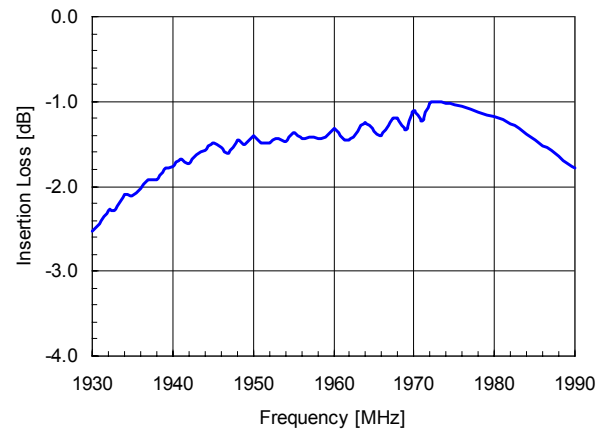
Figure 4. Ant-Rx insertion loss
