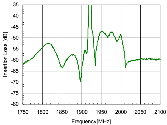
Figure 7. Tx-Rx isolation
