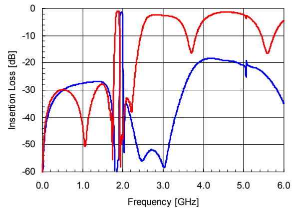
Figure 10. Tx-Ant and Ant-Rx wideband insertion loss
