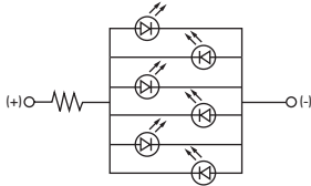
AT621 Bicolor LED 5-volt 6-element with Resistor
