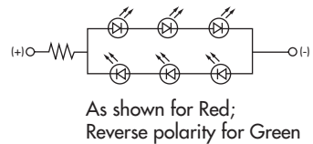
AT621 Bicolor LED 12 & 24-volt 6-element with Resistor
